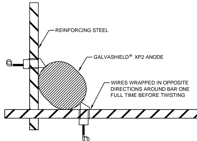
PLAN OF TYPICAL INSTALLATION AT REBAR INTERSECTION
