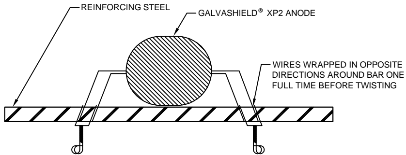
PLAN OF TYPICAL INSTALLATION TO SIDE OF REBAR
