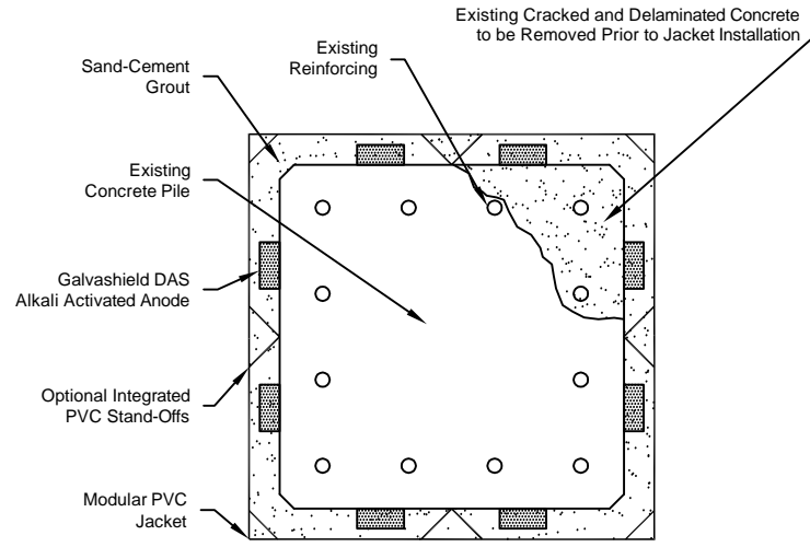
GALVASHIELD DAS JACKET CROSS-SECTION N.T.S.
