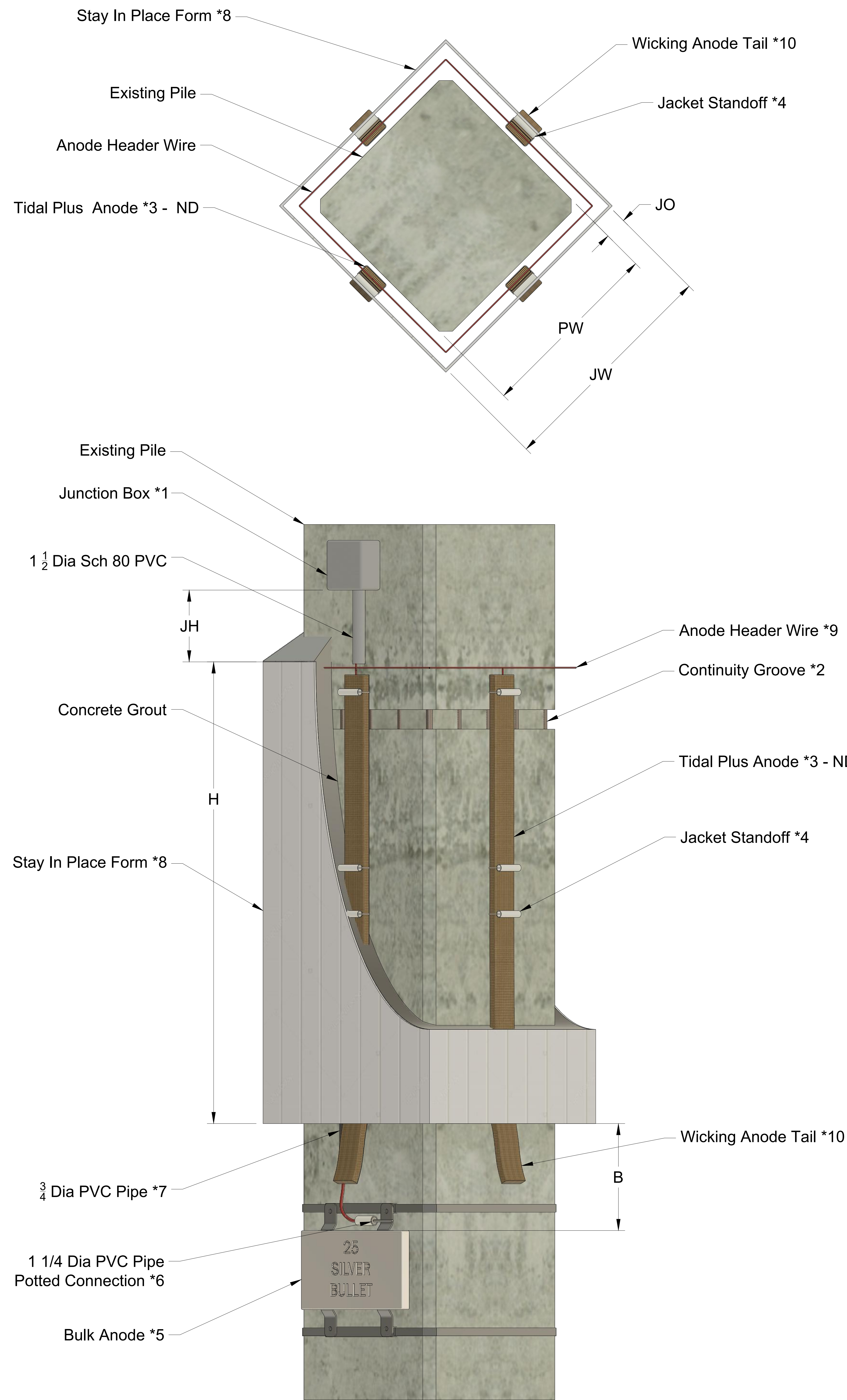
ELEVATION VIEW
