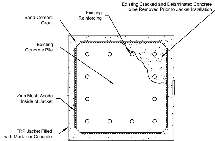
GALVASHIELD TIDAL JACKET CROSS-SECTION
