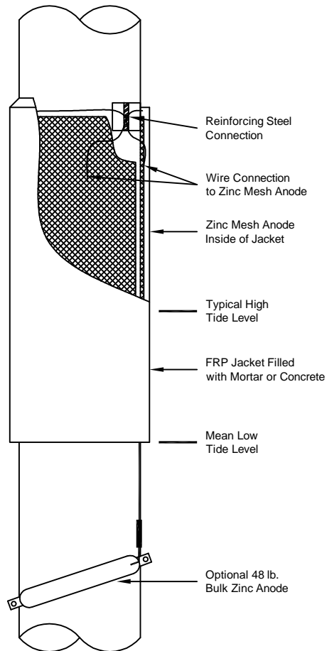
GALVASHIELD TIDAL JACKET ELEVATION
